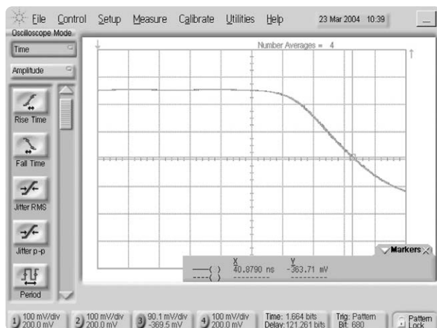
Figure 23. Worst case Late edge view
