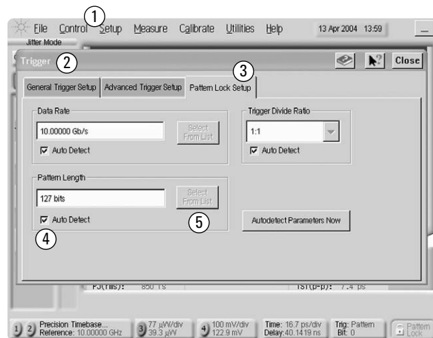
Figure 10. Jitter setup menu for customizing the measurement process
