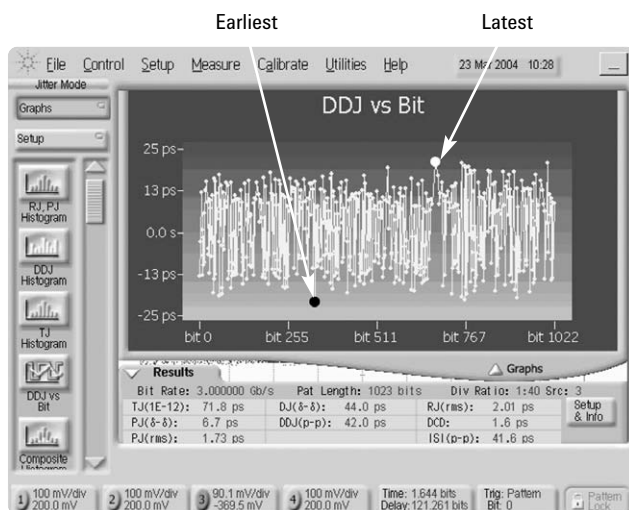
Figure 20. Troubleshooting DDJ
