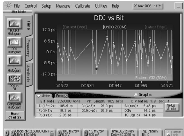
Figure 18. Increased resolution for DDJ versus bit
