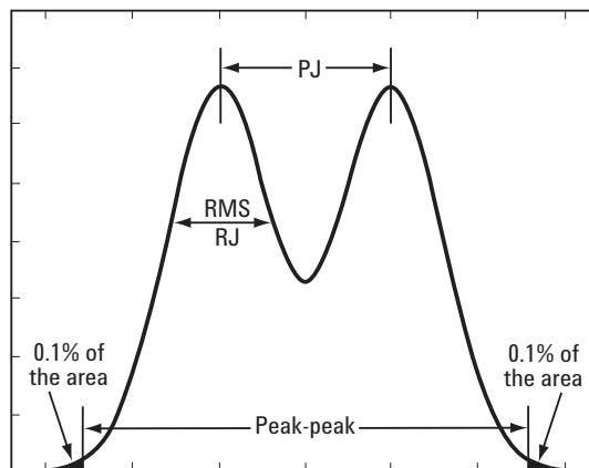
Figure 7. The dual-Dirac delta jitter model
