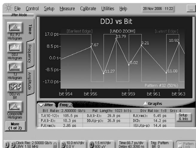
Figure 19. Zooming in on the DDJ versus bit display
