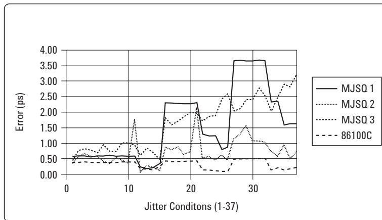
Figure 32. Error in measured RJ versus DCD/ISI/PJ/RJ condition
