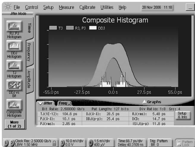
Figure 16. Composite jitter histogram
