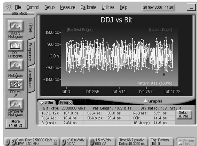
Figure 17. DDJ versus bit display
