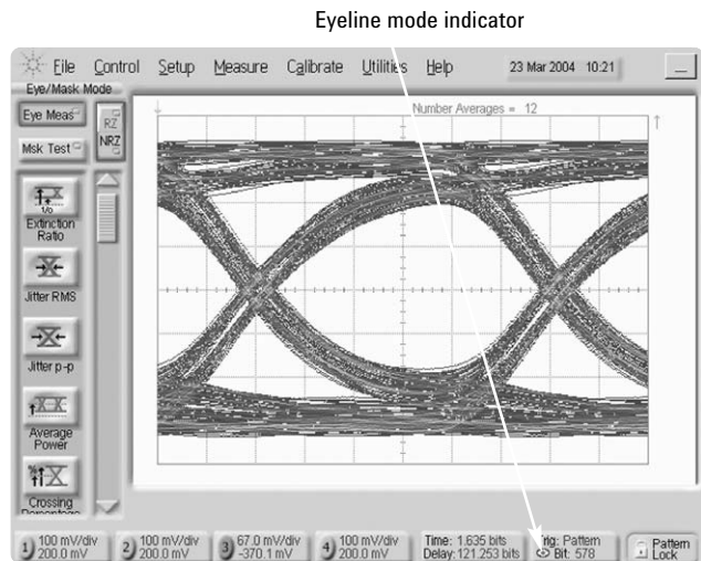
Figure 27. Eyeline view of eye diagram
