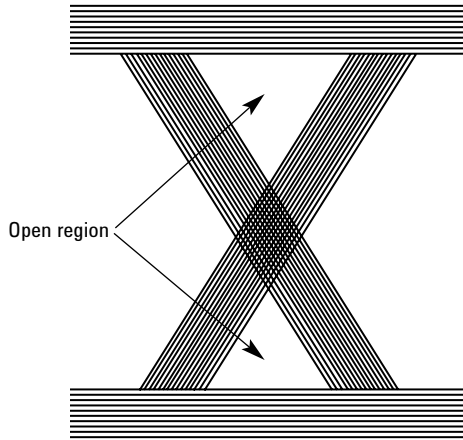
Figure 31: Allowable jitter (PJ, RJ)
