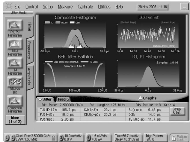
Figure 8. Combined histograms and tabular results
