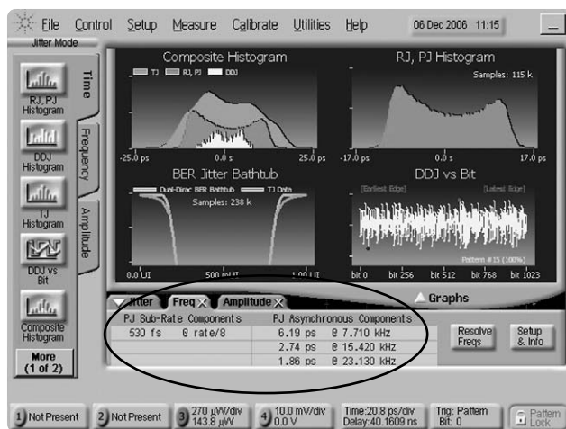
Figure 28: Isolating periodic jitter components
