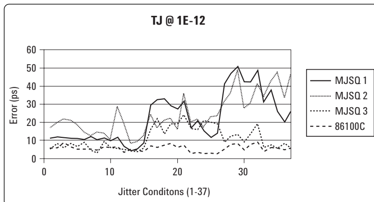
Figure 33. Error in measured TJ versus DCD/ISI/PJ/RJ condition
