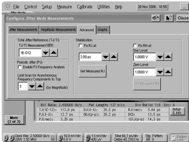
Figure 15. Setup for total jitter bathtub
