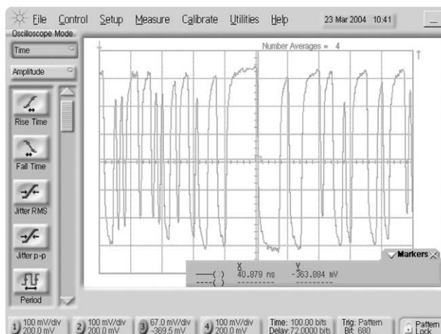
Figure 24. Worst case Late edge within pattern
