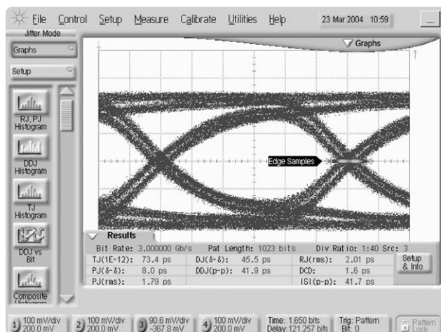
Figure 22. Time position of triggered bit
