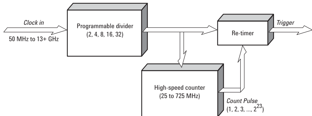
Figure 4: 86100C conceptual diagram for internally deriving a pattern trigger
