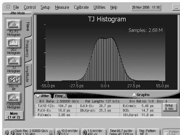
Figure 13. Total jitter histogram
