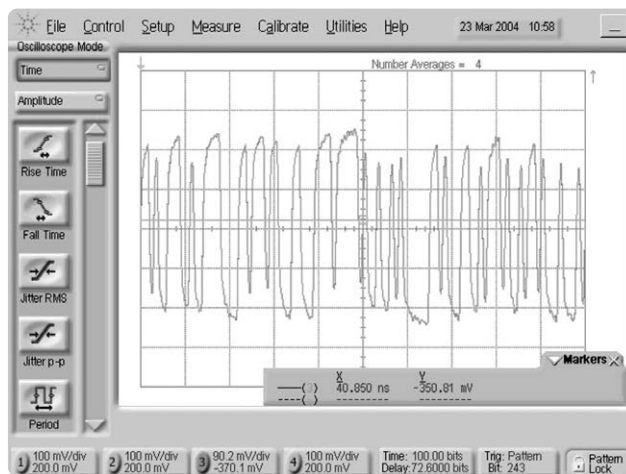
Figure 26. Worst case Early edge within pattern
