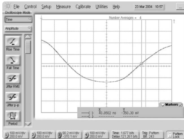
Figure 25. Worst case Early edge
