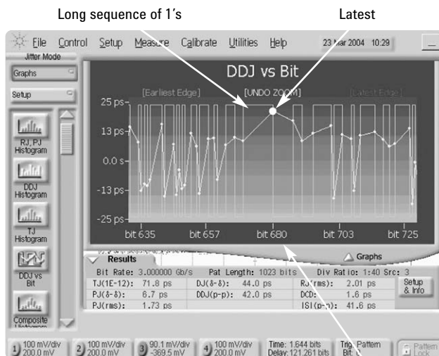
Figure 21. Worst case DDJ
