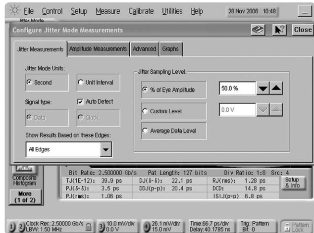
Figure 10. Jitter setup menu for customizing the measurement process
