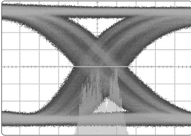
Figure 3. Jitter observed through the histogram of the eye diagram crossing point
