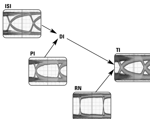
Figure 2. Interference is composed of several types of amplitude impairment
