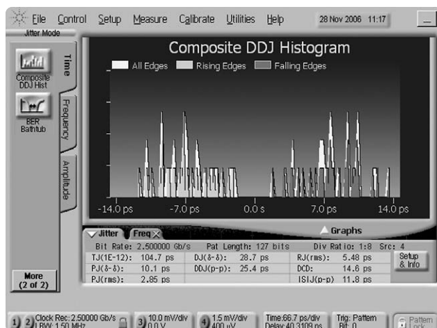
Figure 12. DDJ histograms
