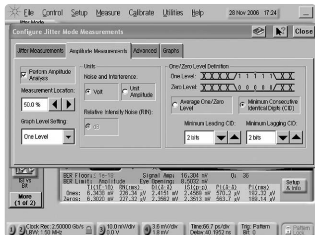
Figure 29: Setup page for amplitude interference measurements
