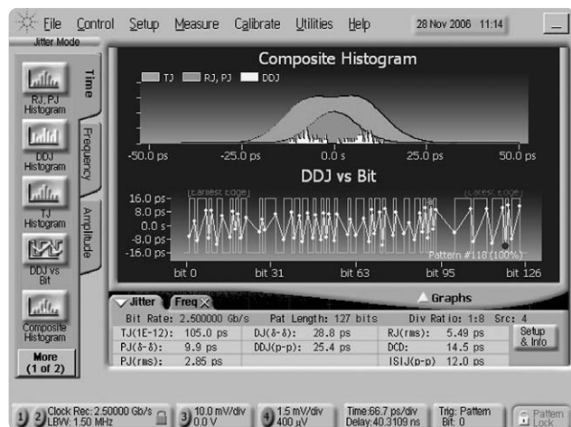
Figure 6. DDJ, RJ/PJ, and TJ histograms with DDJ versus bit - split display
