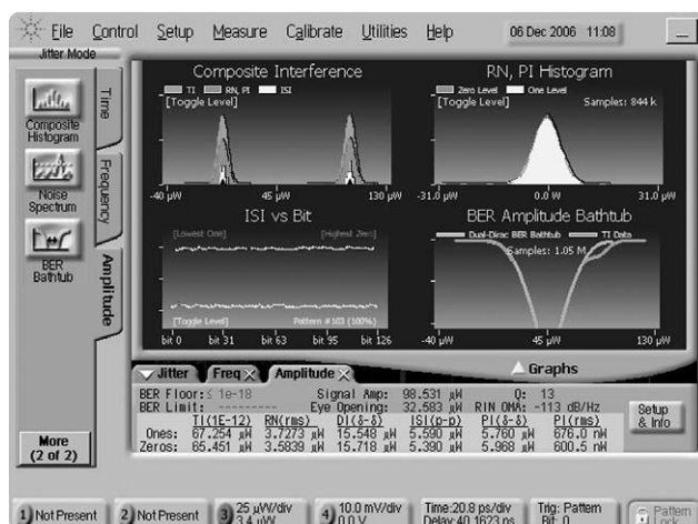
Figure 30: Total interference is composed of several types of interference
