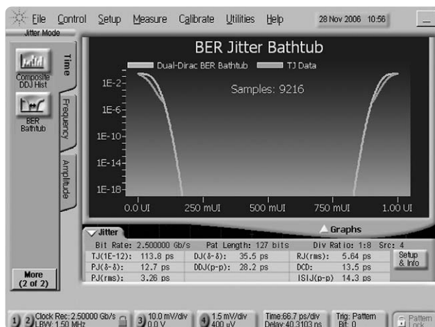
Figure 14. Bathtub curve for total jitter
