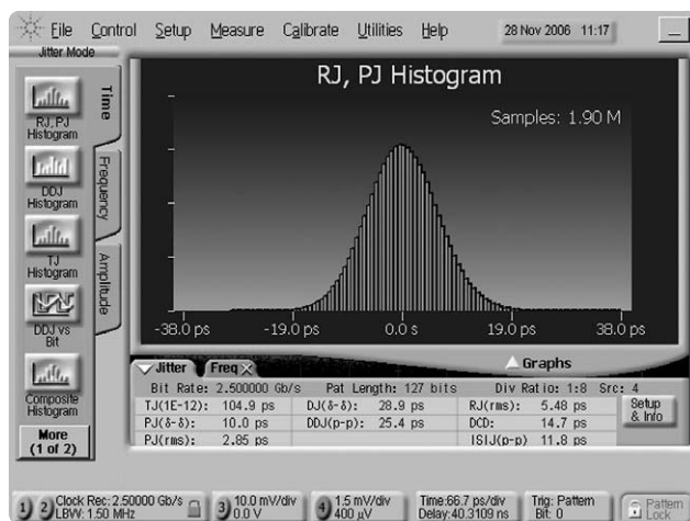
Figure 11. RJ, PJ histogram display
