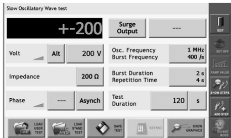
Slow Damped Oscillatory Wave test window
