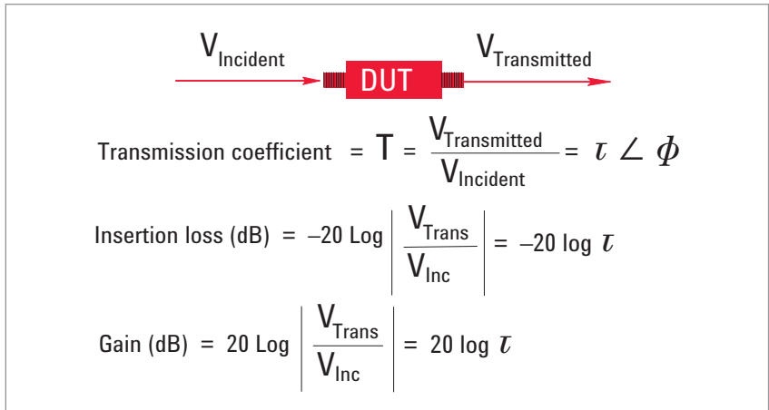
Figure 12. Transmission parameters
