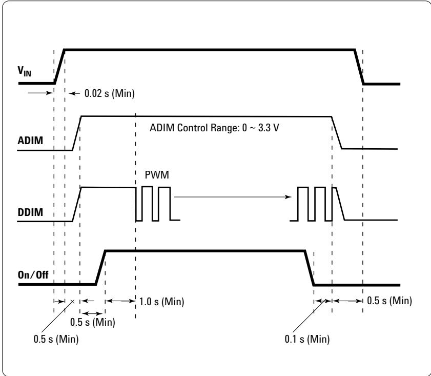
Figure 1. Typical Inverter Input Timing Graph
