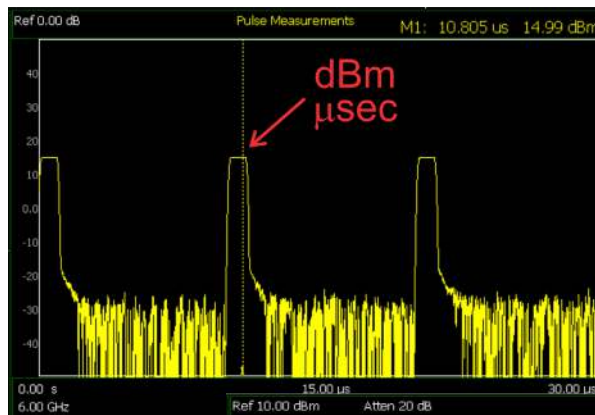
(a) Absolute time domain measurement using peak power meter
