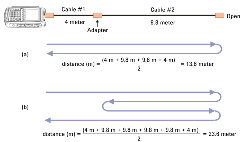
Figure 11. Signal propagation paths between FieldFox and an open-ended cable; (a) signal reflection from the open end, (b) double reflection from the open end and the adapter.
