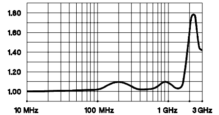
VSWR (75 \Omega )
