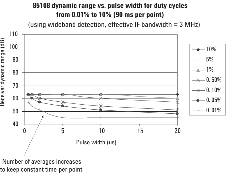
Figure 47. 85108A dynamic range versus pulse width for various duty cycles
