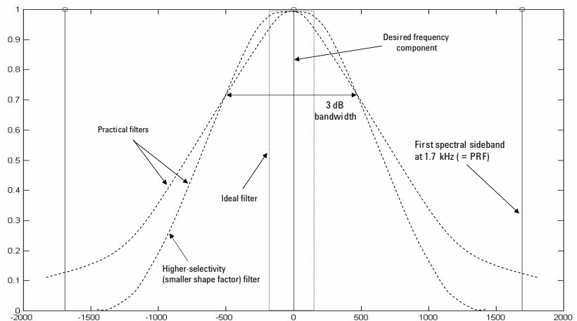
Figure 23. A zoomed-in view of the example pulse spectrum showing ideal and practical filter responses
