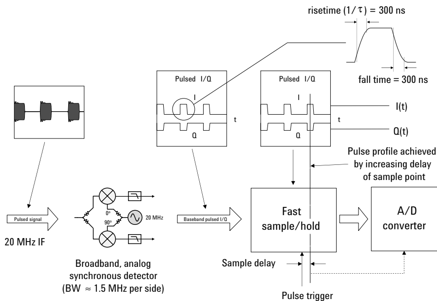
Figure 12. Time-domain view of wideband detection in the 85108 pulsed-RF system
