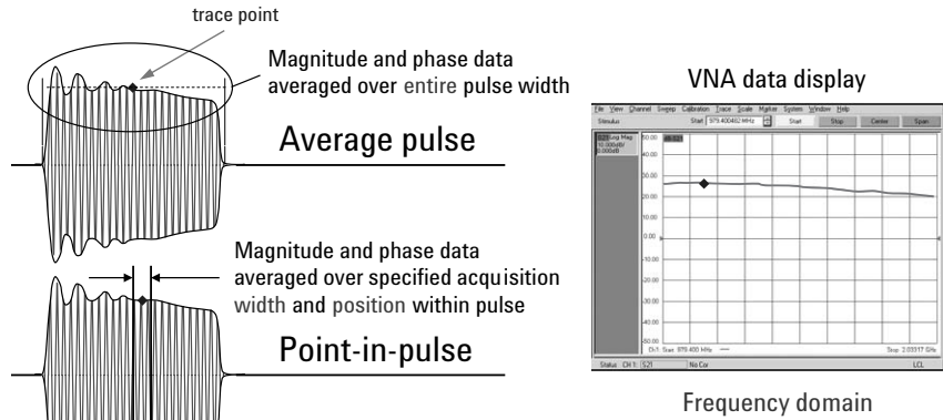
Figure 3. Average and point-in-pulse measurements
