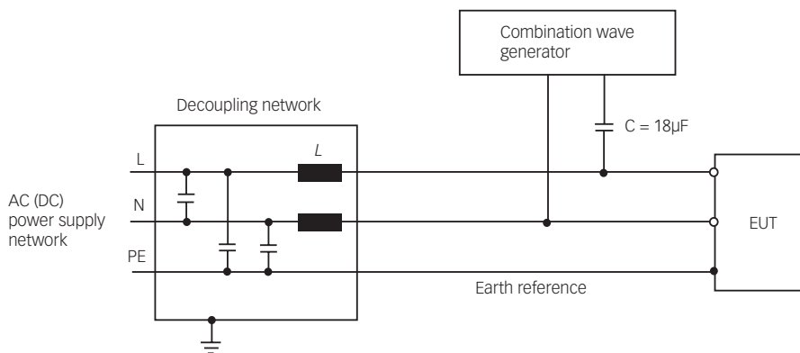
Schematic of a surge CDN (single phase)
