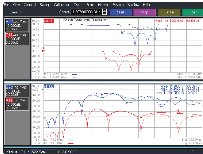
Figure 17. The Rx side of the filter is being tuned here. The upper plot shows the S11 and S22 of the filter; each set to a different center frequency appropriate for the first and last resonator. The lowest plot shows the null from each resonator.
