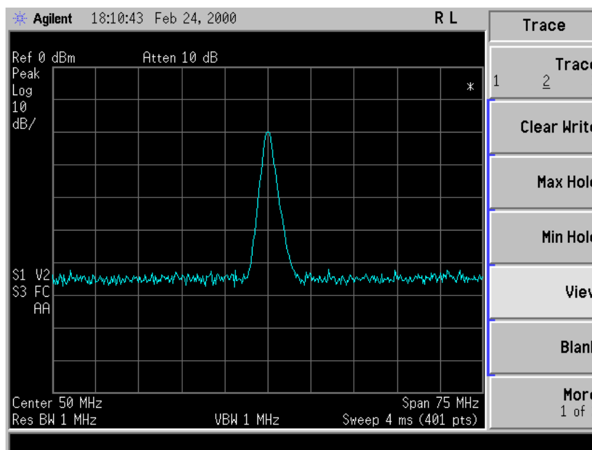
Figure 4-7. Verifying Trace 1
