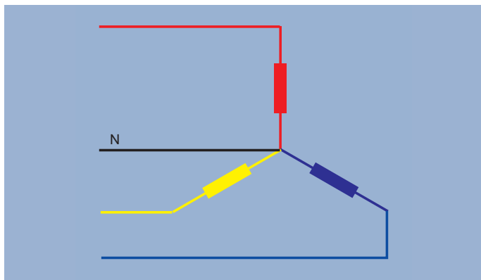
Figure 5. Wye or star connection - three-phase, four wires.
