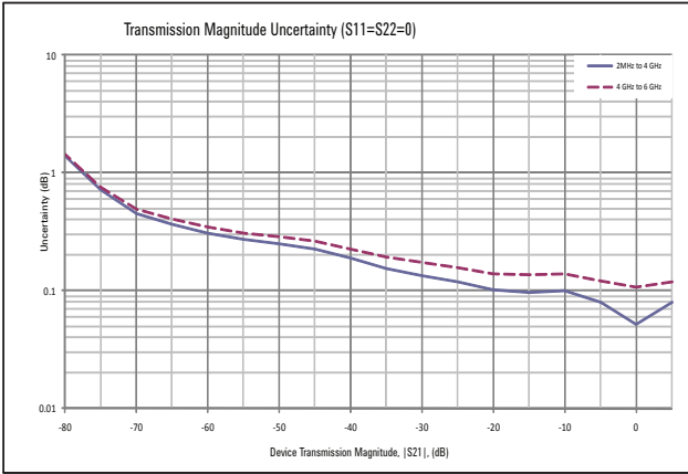
Figure 5: Transmission uncertainty
