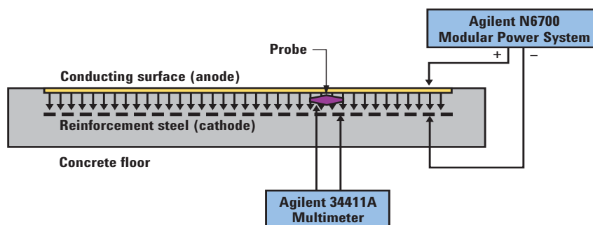
Figure 1. Cathodic protection (example)
