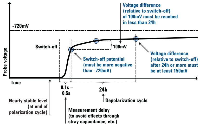
Figure 3. Interpretation of measurement results (example)
