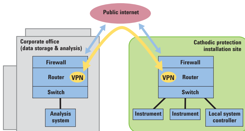
Figure 4. VPN and IPSec enable secure, encrypted data exchange via the public internet
