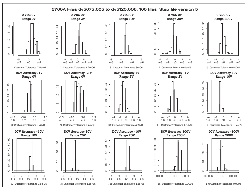
Figure 10. Measured production test results on a Fluke 5700A Calibrator
