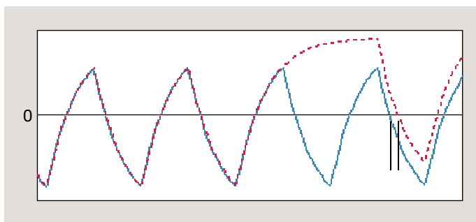
Figure 4.2.4b. Limited Bandpass One Source of Data Dependent Jitter.
