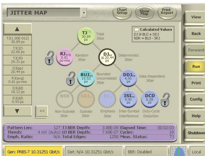
Figure 2.4d. BERT with Jitter Values on a Jitter Map.
