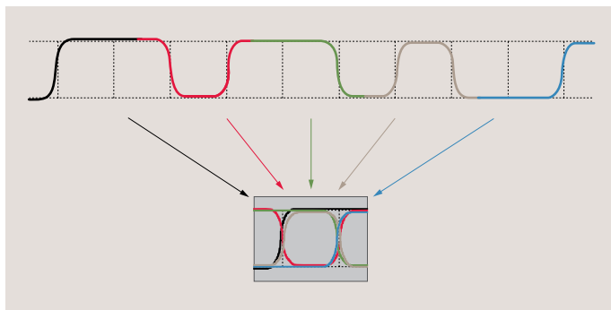
Figure 3.5a. Constructing a Real-Time Eye Diagram.
