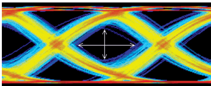
Figure 3.5b. A Waveform Database with Color Gradation.
