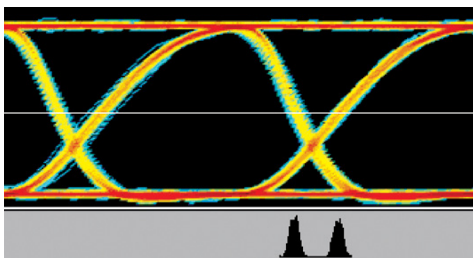
Figure 4.2.5a. Duty Cycle Distortion Caused by Non-symmetrical Rise/Fall Times.
