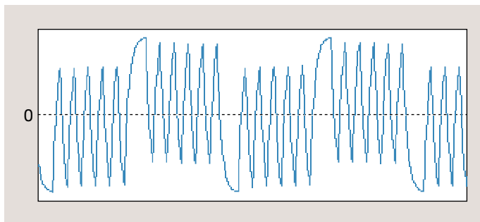
Figure 4.2.4a. Data Signal with Data Dependent Jitter.
