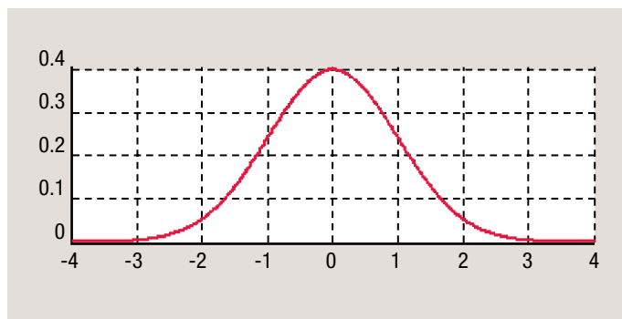
Figure 4.2.1a. Gaussian Distribution.
