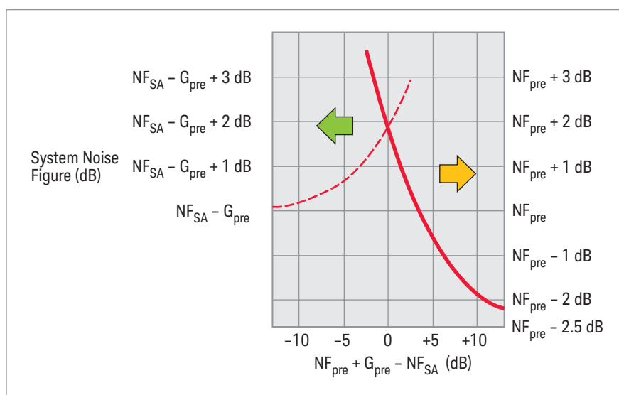
Figure 5-6. System noise figure for sinusoidal signals
