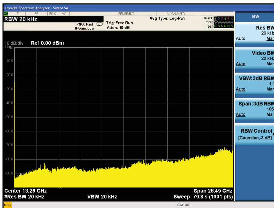
Figure 2-14a. Full span sweep speed, RBW of 20 kHz, without Option FS1
