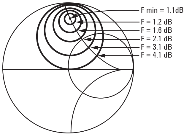
Figure 2-2. Noise circles
